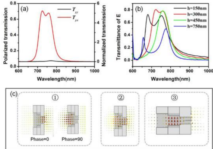
Fig. 3. Numerical results of transmission properties for 90^\circ rotation structure. (a) Transmission spectra detected in x - and y -polarization under y -polarized incidence (here h=300\text{nm} ). (b) Transmittance of E_x for different total thicknesses, as h=150\text{nm} , 300\text{nm} , 450\text{nm} , 750\text{nm} , respectively. (c) E field Distributions of distinct modes marked out in (b).
