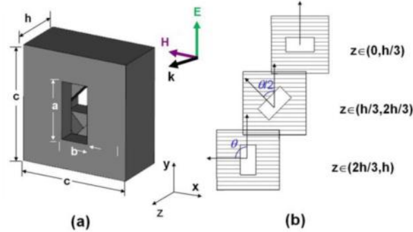
Fig. 1. (a) Unit cell of proposed stereo plasmonic waveguide array with structural parameters of a=300\text{nm} , b=150\text{nm} , c=600\text{nm} , h=300\text{nm} , and \theta=90^\circ . (b) Cross section of stereo structure at three layers respectively.
