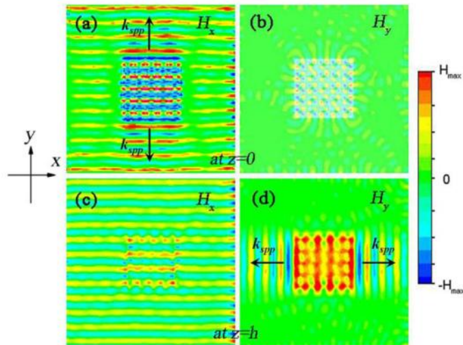
Fig. 4. Magnetic field distributions on the metal surfaces of a stereo structure containing 5 \times 5 period array with h=300\text{nm} and \theta=90^\circ at \lambda=769\text{nm} : (a) H_x and (b) H_y at incident side z=0 , (c) H_x and (d) H_y at transmission side z=h , where H_{\max}=0.002\text{A/m} .
