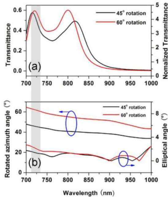
Fig. 2. Numerical result of polarization control of stereo structures with different rotation angles of 45^\circ and 60^\circ . (a) Transmission spectra with polarization perpendicular to long axis of last layer. (b) Spectra of the corresponding rotated azimuth angle and ellipticity angle.
