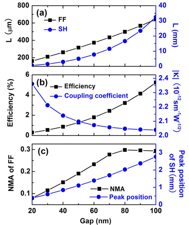
Fig. 3. (Color online) (a) Propagation length ( L ), (b) SHG efficiency and coupling coefficient ( |\kappa| ), (c) normalized mode area (NMA) of FF and peak position of SH as functions of the gap thickness.
