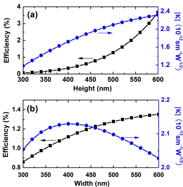
Fig. 4. (Color online) SHG efficiency and coupling coefficient versus (a) height and (b) width of the rectangular \text{LiNbO}_3 waveguide.
