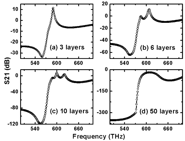
Fig. 3. Transition of the left-handed transmission with stacked metallic layers at the lasing gain coefficient ( 1.09 \times 10^4 \text{ cm}^{-1} ) of the double-layer fishnet structure in Fig. 2.
