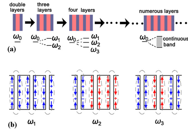
Fig. 4. (Color online.) (a) Split resonance frequencies for the plasmon hybridization in layer-to-layer coupling fishnet metamaterials. (b) Three hybridization modes for a four-layer fishnet metamaterial. Arrows denote the induced surface current, while “+” and “−” present the locations of charge accumulation.
