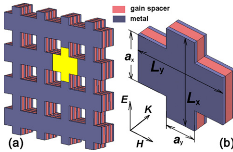
Fig. 1. (Color online.) The schematic illustration of the bulk metallic fishnet metamaterial with active layer as the spacer. (a) Bulk fishnet metamaterial with four-layer metallic fishnet structures, the yellow area indicates an xy -face of the selected unit cell. (b) The unit scales for the fishnet metamaterial.
